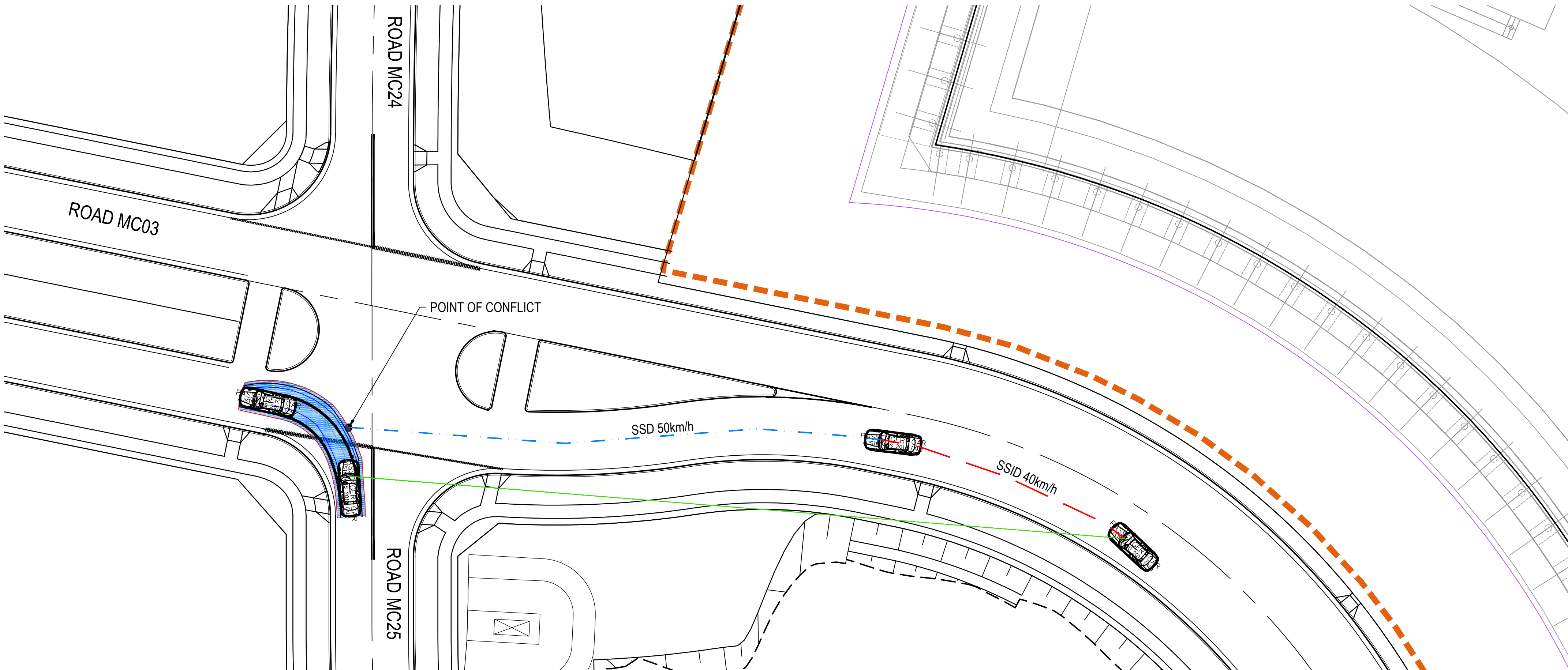
ROAD MC25 - ROAD MC03 INTERSECTION 7 APPROACH SIGHT DISTANCE SCALE 1 : 250
